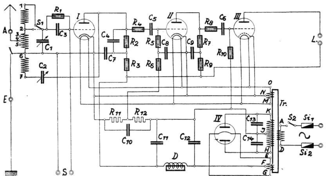
Principe-schema
